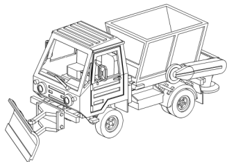
M 25 sypač / spreader with blade
